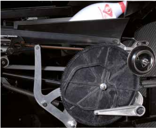
EDGE Distributor Cam for Durabin
